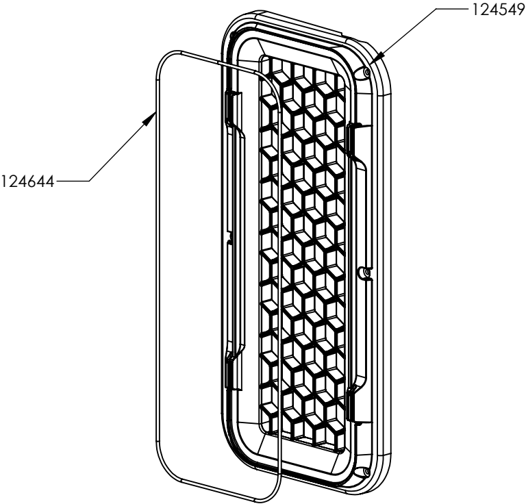
OUTLET GRILL ASSEMBLY
