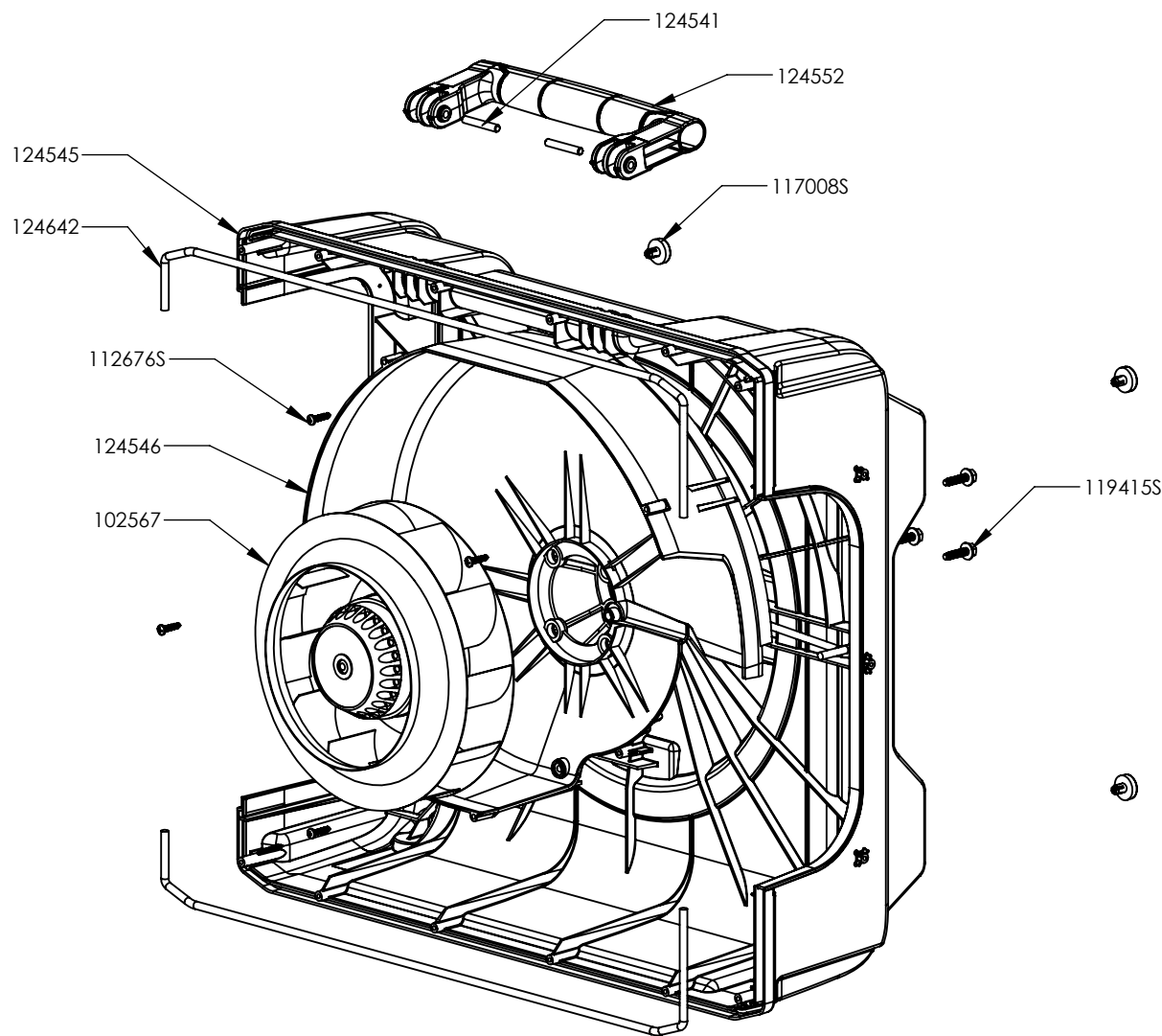
REAR PANEL ASSEMBLY
