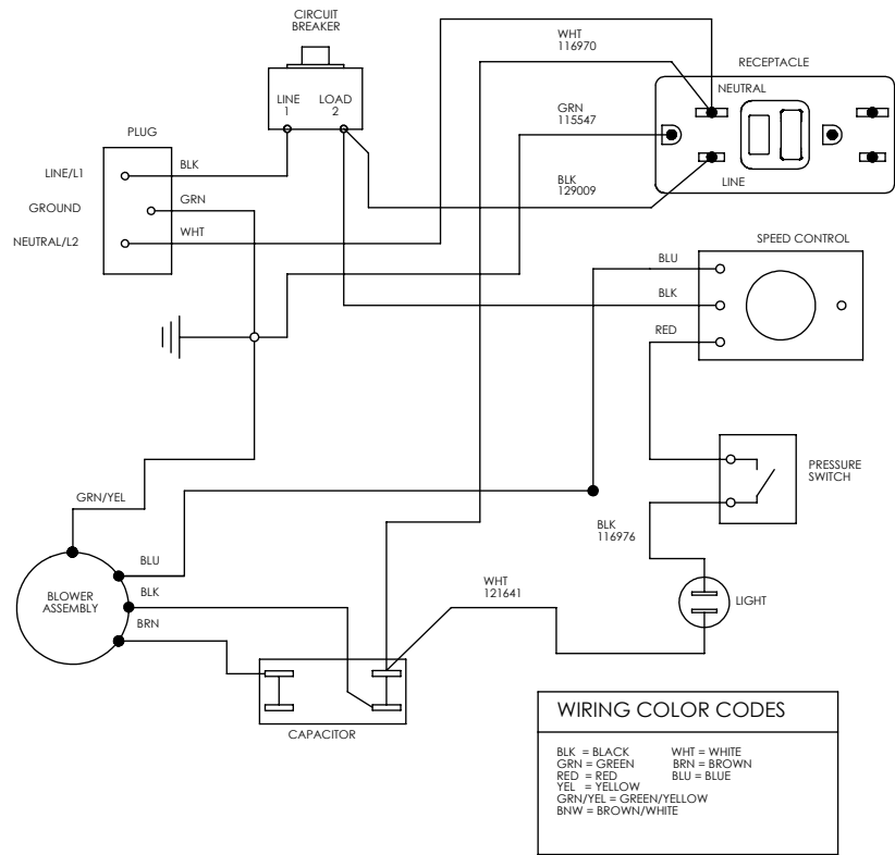
WIRING SCHEMATIC - DEFENDAIR HEPA 700 115V
