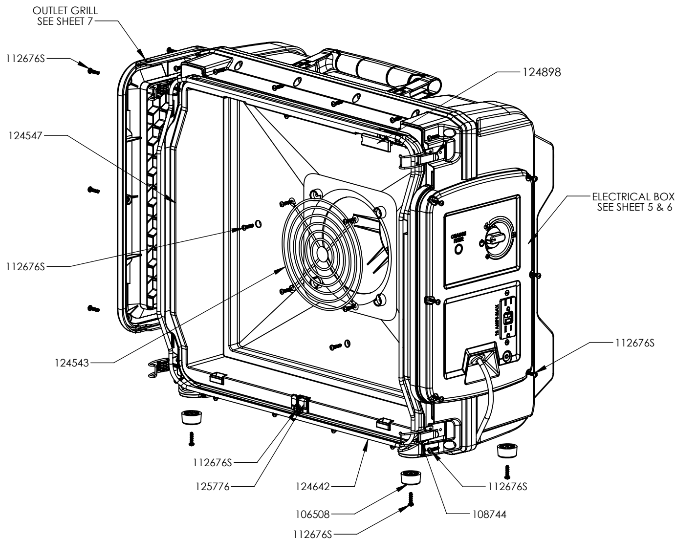
PLENUM ASSEMBLY DETAIL
